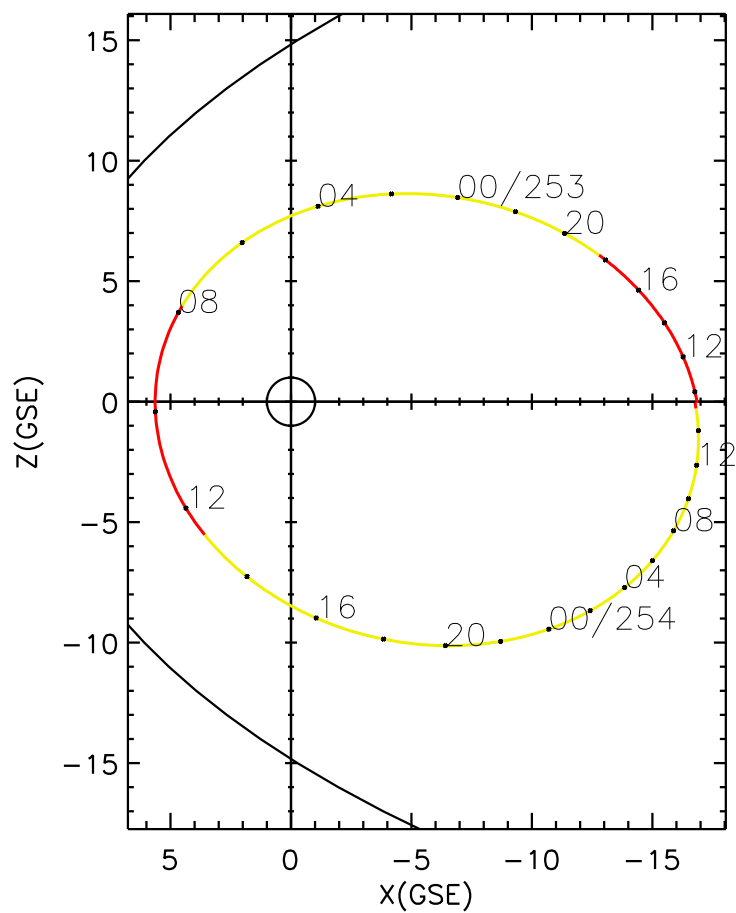
CLUSTER 2 orbit 2017 252 (09/09) 09:21 UT to 2017 254 (09/11) 15:36 UT
