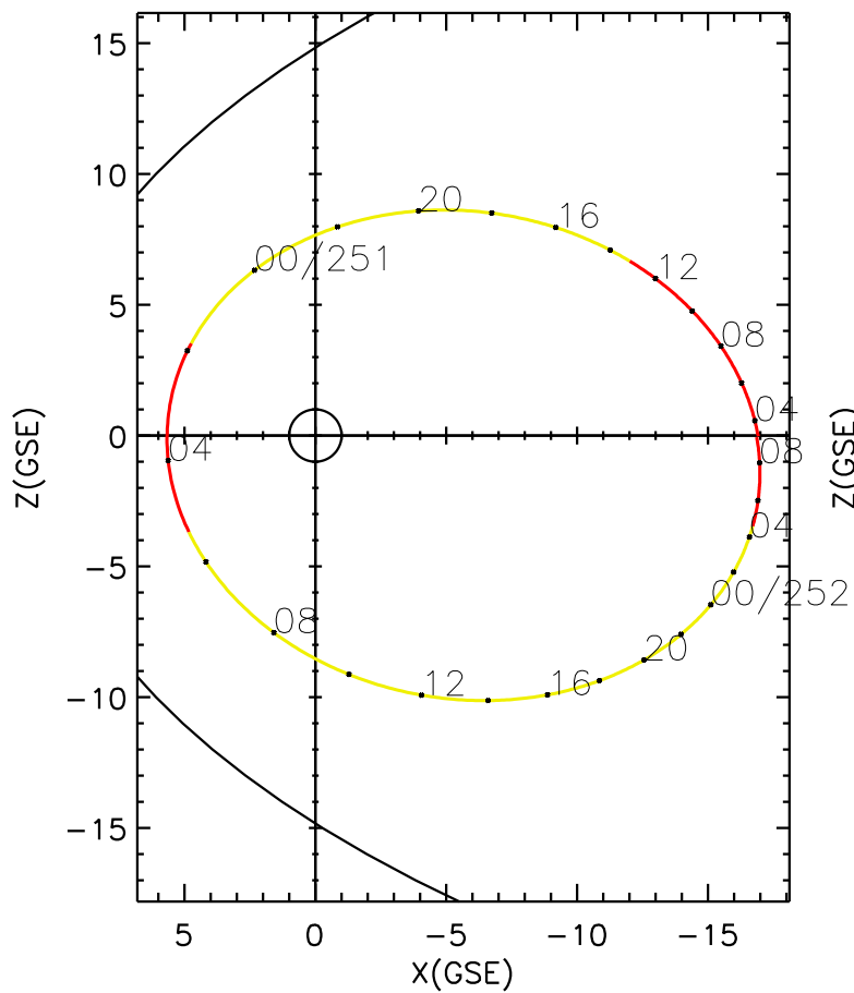
CLUSTER 2 orbit 2017 250 (09/07) 03:11 UT to 2017 252 (09/09) 09:21 UT
