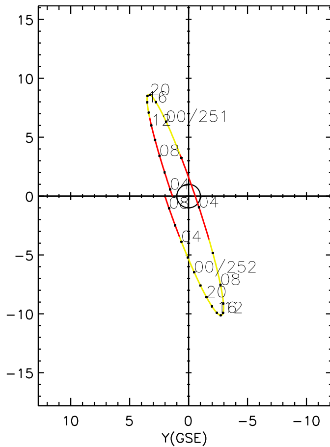
CLUSTER 2 orbit 2017 250 (09/07) 03:11 UT to 2017 252 (09/09) 09:21 UT
