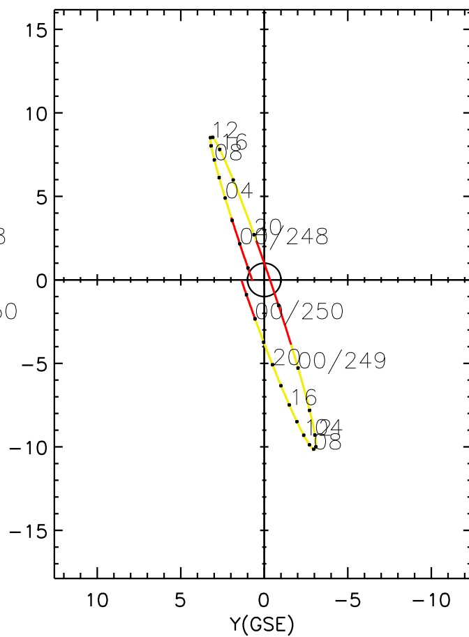
CLUSTER 2 orbit 2017 247 (09/04) 20:56 UT to 2017 250 (09/07) 03:11 UT
