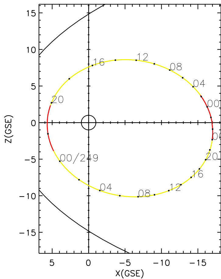
CLUSTER 2 orbit 2017 247 (09/04) 20:56 UT to 2017 250 (09/07) 03:11 UT
