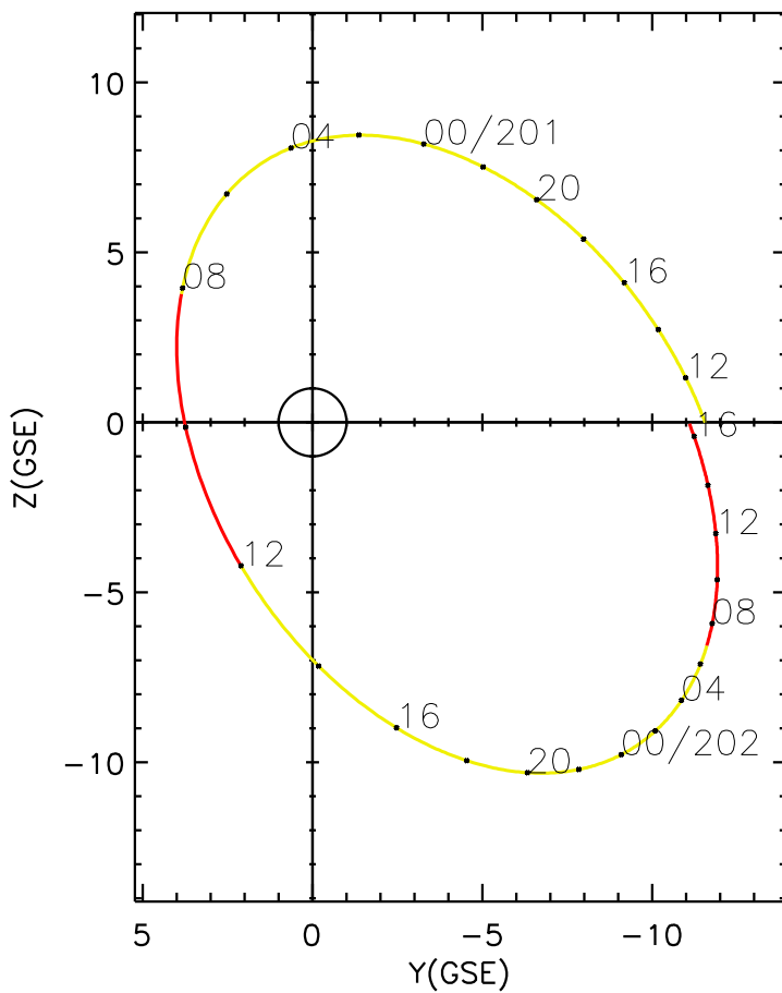
CLUSTER 2 orbit 2017 200 (07/19) 10:11 UT to 2017 202 (07/21) 16:31 UT
