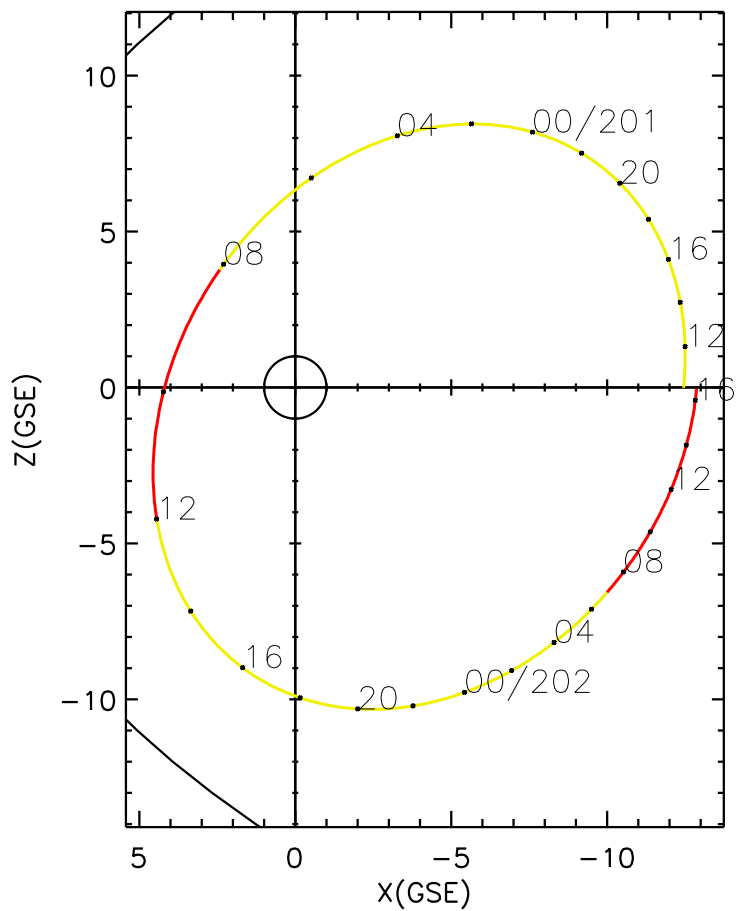
CLUSTER 2 orbit 2017 200 (07/19) 10:11 UT to 2017 202 (07/21) 16:31 UT
