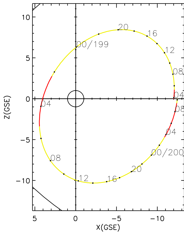
CLUSTER 2 orbit 2017 198 (07/17) 03:46 UT to 2017 200 (07/19) 10:11 UT
