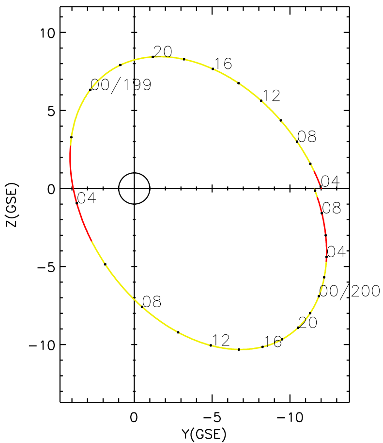
CLUSTER 2 orbit 2017 198 (07/17) 03:46 UT to 2017 200 (07/19) 10:11 UT
