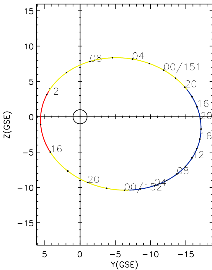
CLUSTER 2 orbit 2017 150 (05/30) 14:01 UT to 2017 152 (06/01) 20:21 UT
