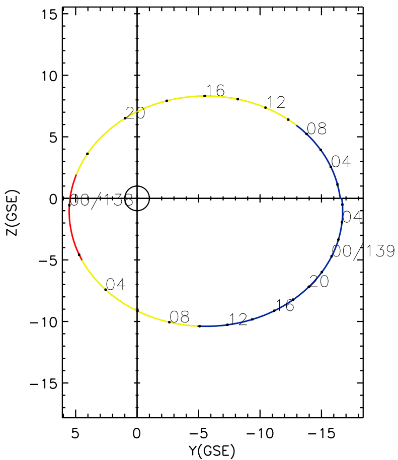
CLUSTER 2 orbit 2017 137 (05/17) 00:21 UT to 2017 139 (05/19) 06:41 UT
