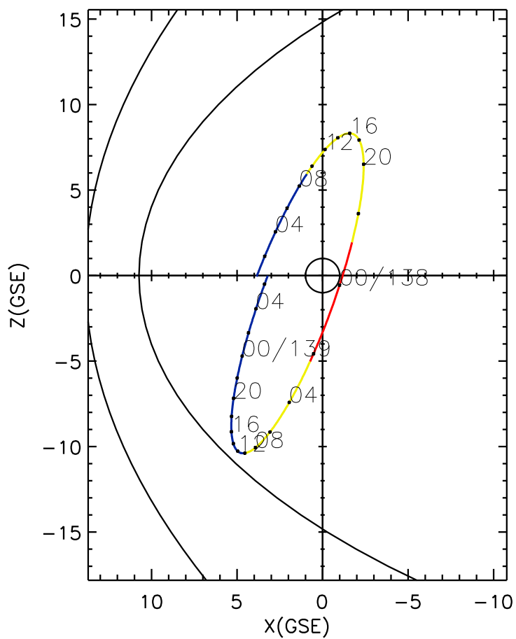
CLUSTER 2 orbit 2017 137 (05/17) 00:21 UT to 2017 139 (05/19) 06:41 UT
