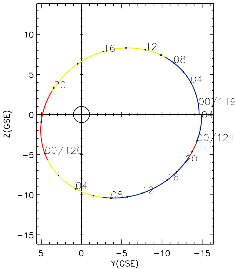
CLUSTER 2 orbit 2017 118 (04/28) 22:16 UT to 2017 121 (05/01) 04:31 UT
