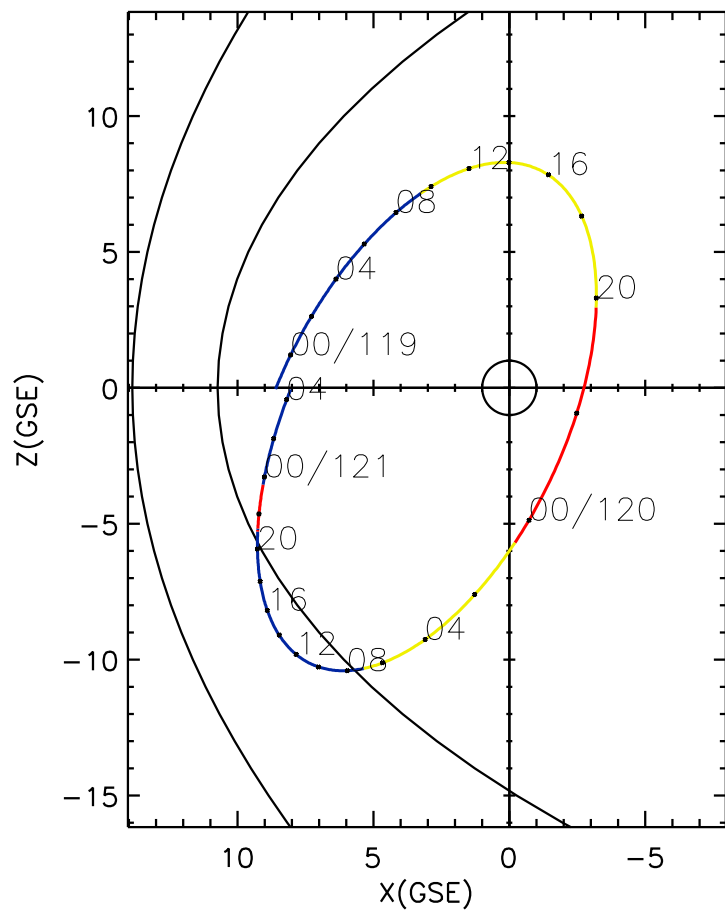
CLUSTER 2 orbit 2017 118 (04/28) 22:16 UT to 2017 121 (05/01) 04:31 UT
