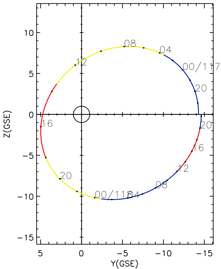
CLUSTER 2 orbit 2017 116 (04/26) 16:01 UT to 2017 118 (04/28) 22:16 UT
