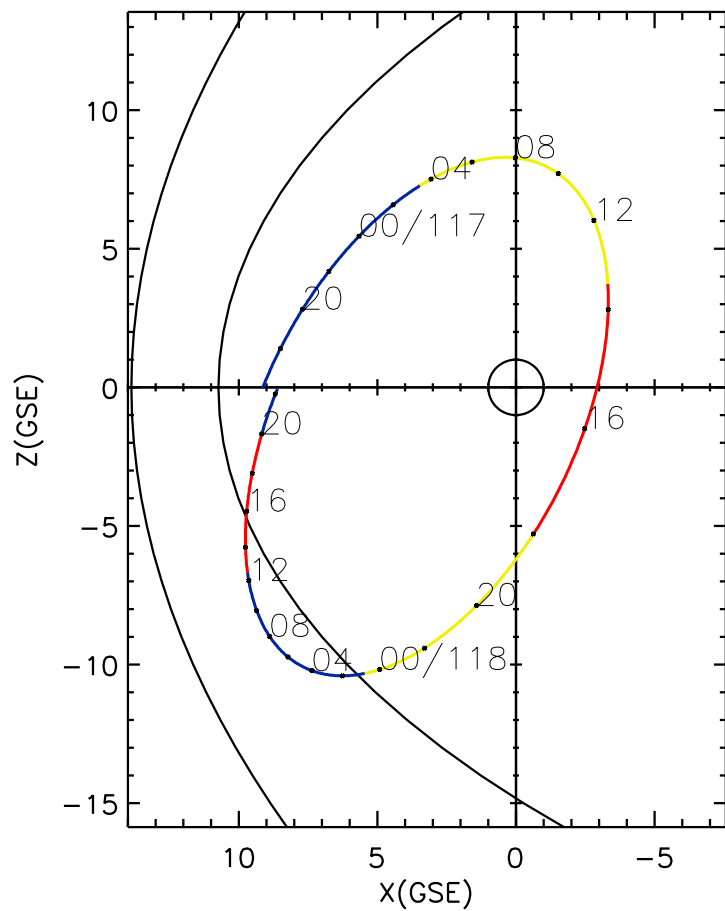
CLUSTER 2 orbit 2017 116 (04/26) 16:01 UT to 2017 118 (04/28) 22:16 UT
