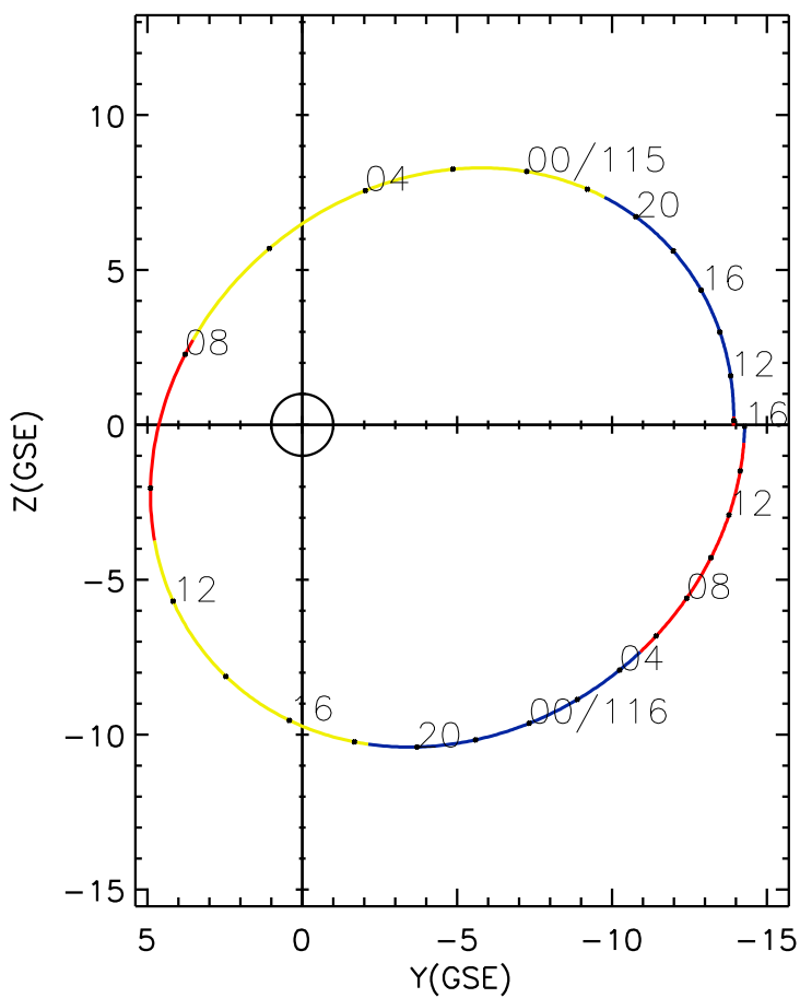
CLUSTER 2 orbit 2017 114 (04/24) 09:46 UT to 2017 116 (04/26) 16:01 UT
