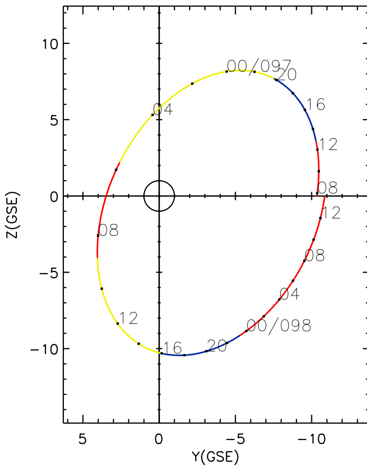
CLUSTER 2 orbit 2017 096 (04/06) 07:41 UT to 2017 098 (04/08) 13:56 UT
