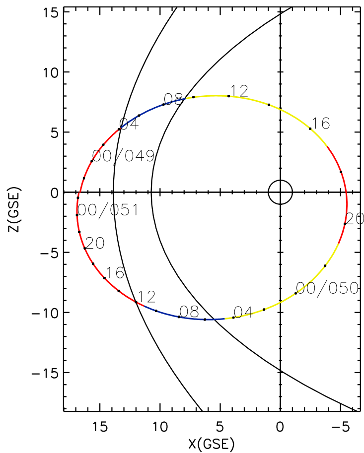
CLUSTER 2 orbit 2017 048 (02/17) 20:21 UT to 2017 051 (02/20) 02:36 UT
