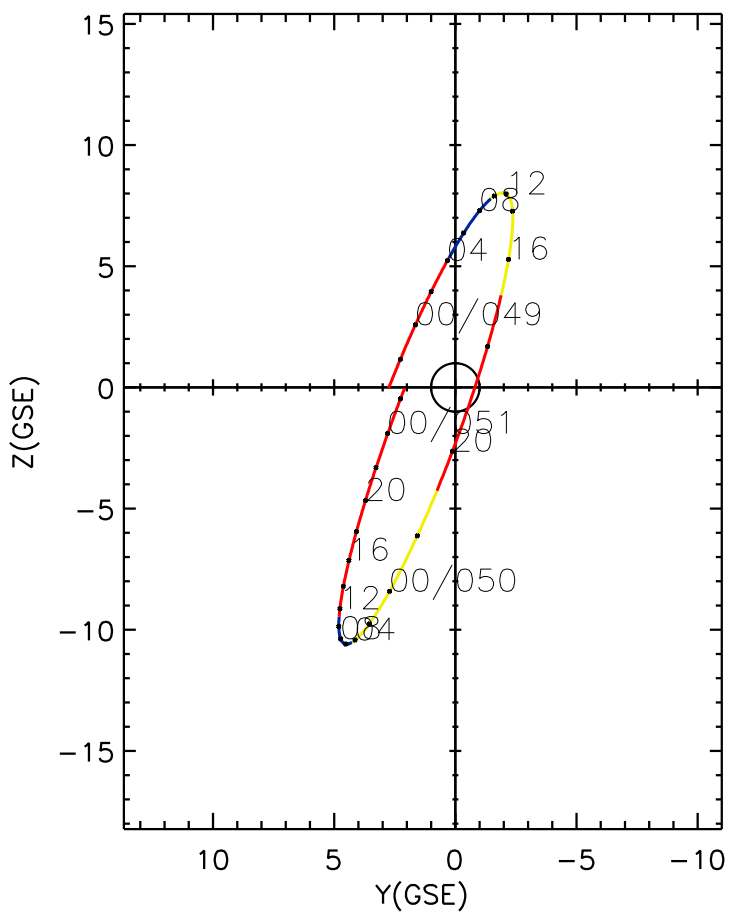
CLUSTER 2 orbit 2017 048 (02/17) 20:21 UT to 2017 051 (02/20) 02:36 UT
