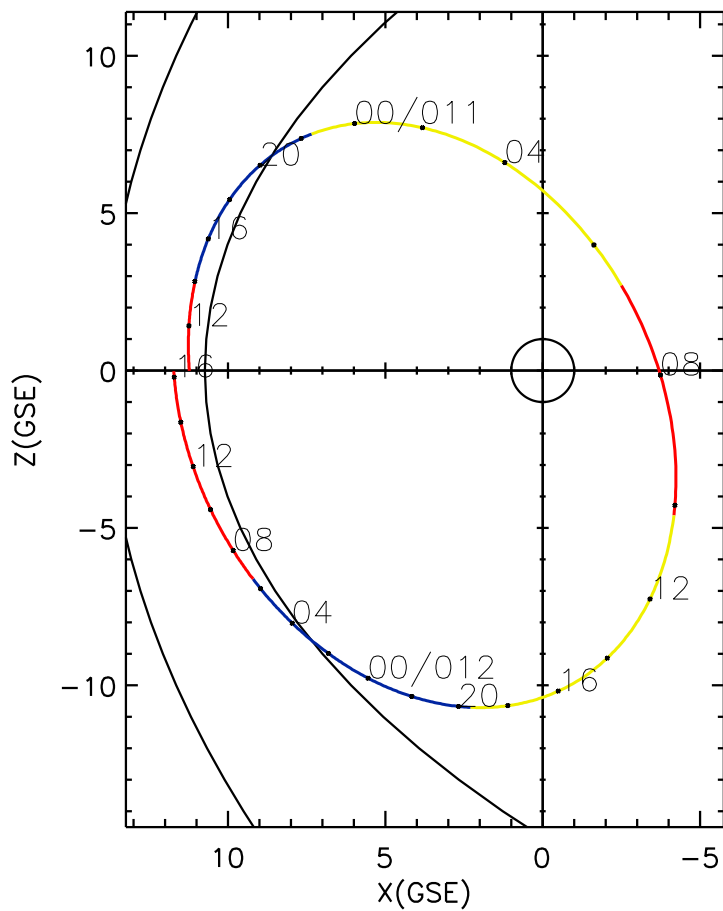
CLUSTER 2 orbit 2017 010 (01/10) 10:01 UT to 2017 012 (01/12) 16:16 UT
