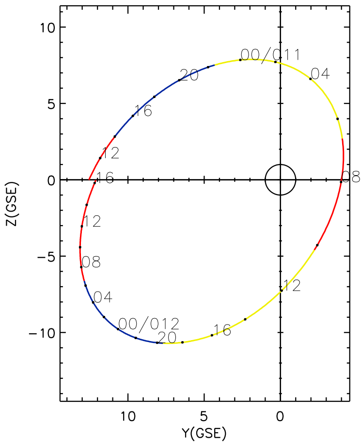
CLUSTER 2 orbit 2017 010 (01/10) 10:01 UT to 2017 012 (01/12) 16:16 UT
