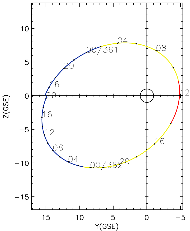
CLUSTER 2 orbit 2016 360 (12/25) 14:11 UT to 2016 362 (12/27) 20:26 UT
