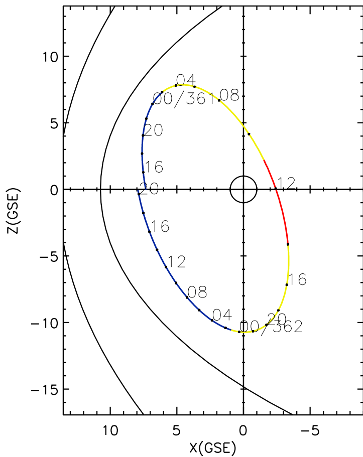
CLUSTER 2 orbit 2016 360 (12/25) 14:11 UT to 2016 362 (12/27) 20:26 UT
