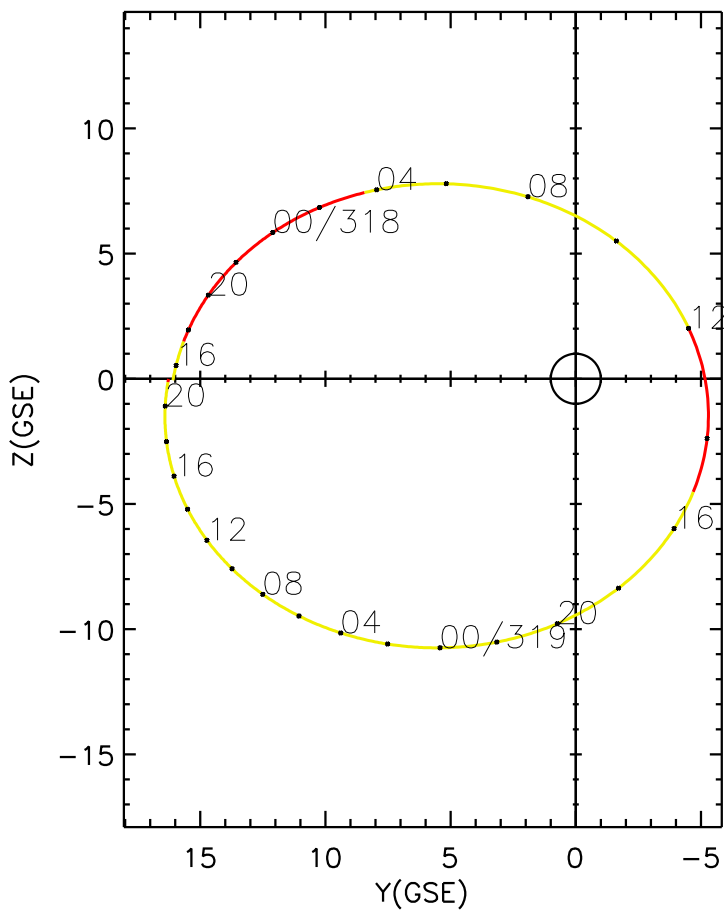
CLUSTER 2 orbit 2016 317 (11/12) 15:11 UT to 2016 319 (11/14) 21:31 UT
