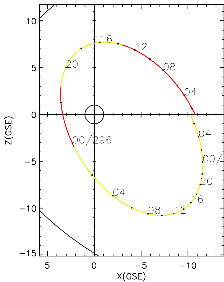
CLUSTER 2 orbit 2016 295 (10/21) 01:06 UT to 2016 297 (10/23) 07:16 UT
