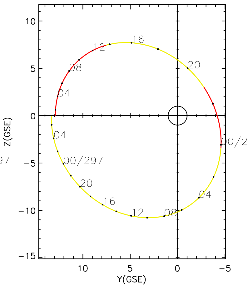
CLUSTER 2 orbit 2016 295 (10/21) 01:06 UT to 2016 297 (10/23) 07:16 UT
