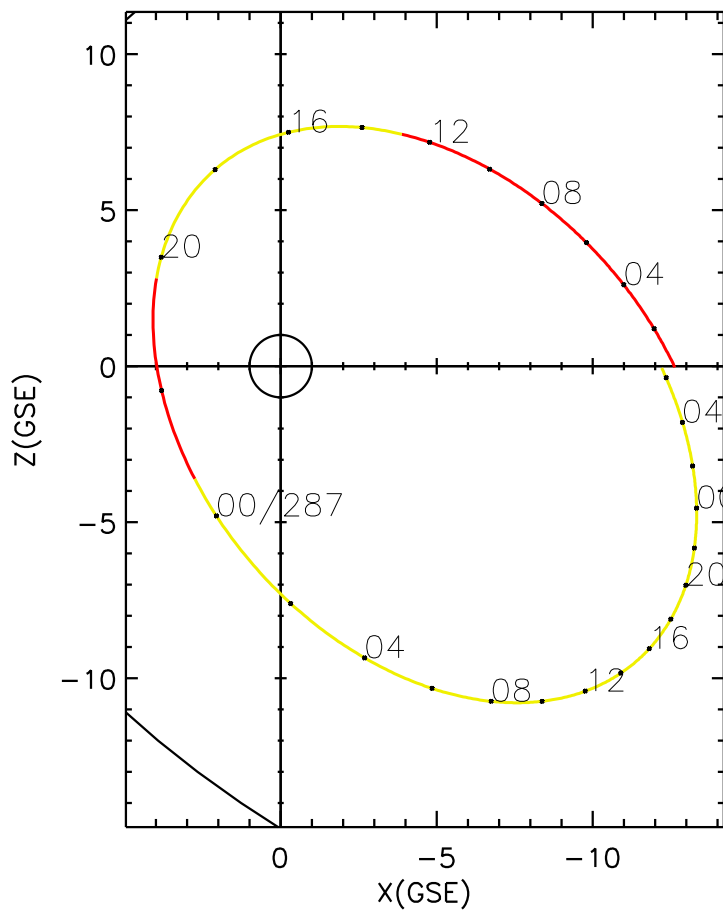
CLUSTER 2 orbit 2016 286 (10/12) 00:16 UT to 2016 288 (10/14) 06:26 UT
