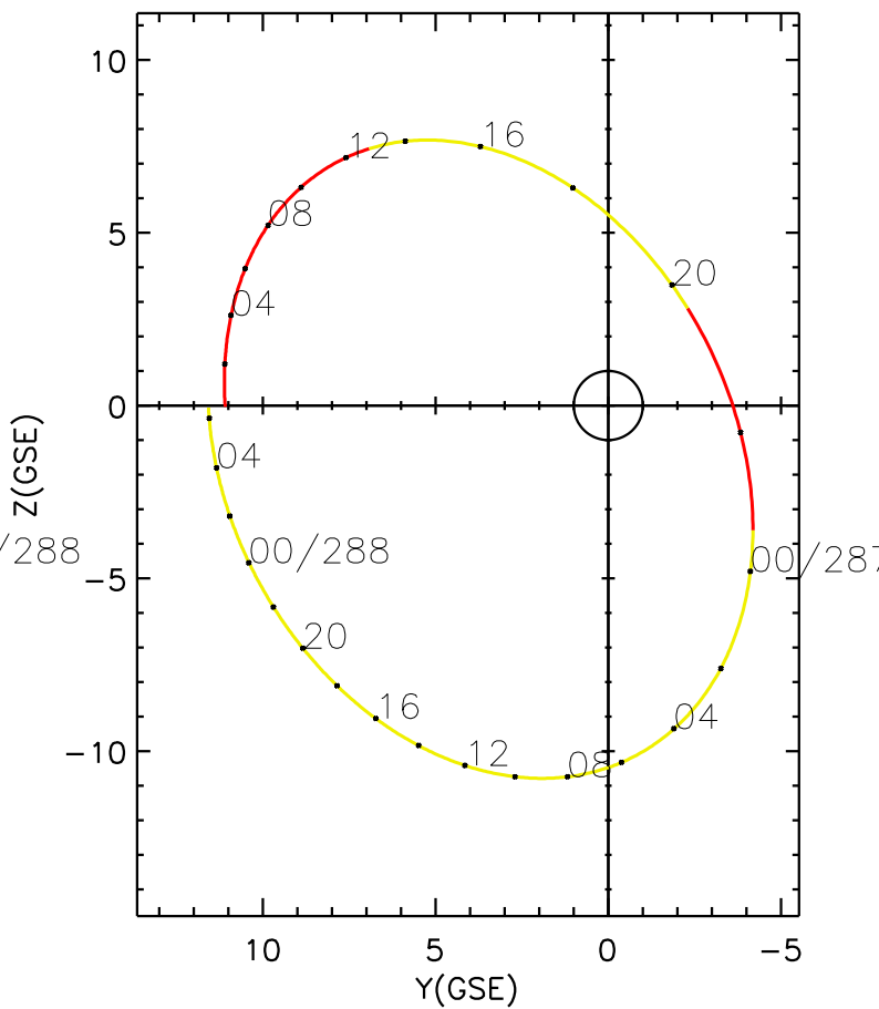
CLUSTER 2 orbit 2016 286 (10/12) 00:16 UT to 2016 288 (10/14) 06:26 UT
