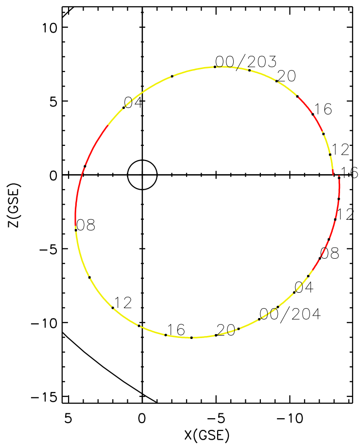
CLUSTER 2 orbit 2016 202 (07/20) 10:01 UT to 2016 204 (07/22) 16:16 UT
