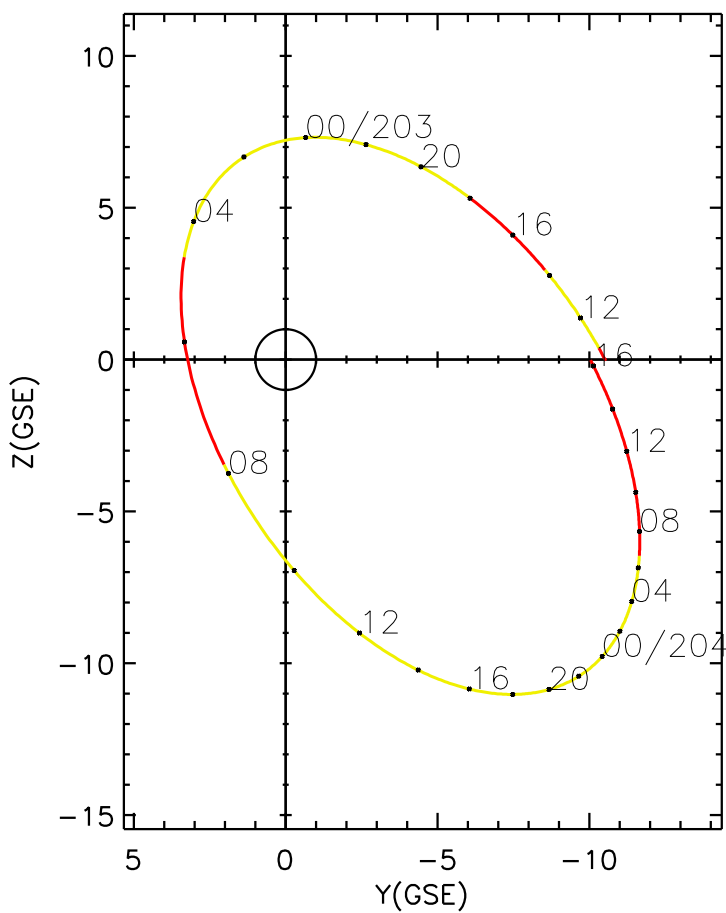
CLUSTER 2 orbit 2016 202 (07/20) 10:01 UT to 2016 204 (07/22) 16:16 UT
