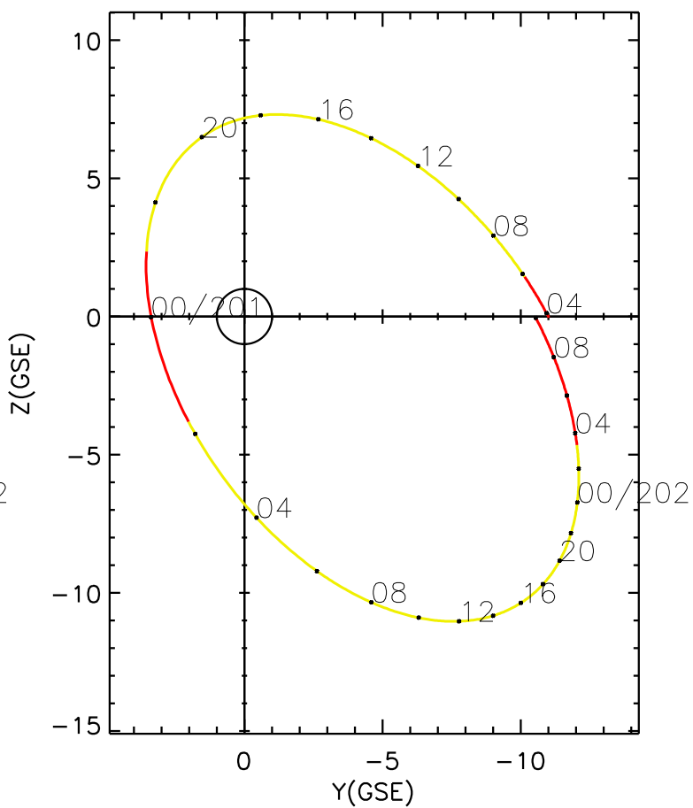
CLUSTER 2 orbit 2016 200 (07/18) 03:46 UT to 2016 202 (07/20) 10:01 UT
