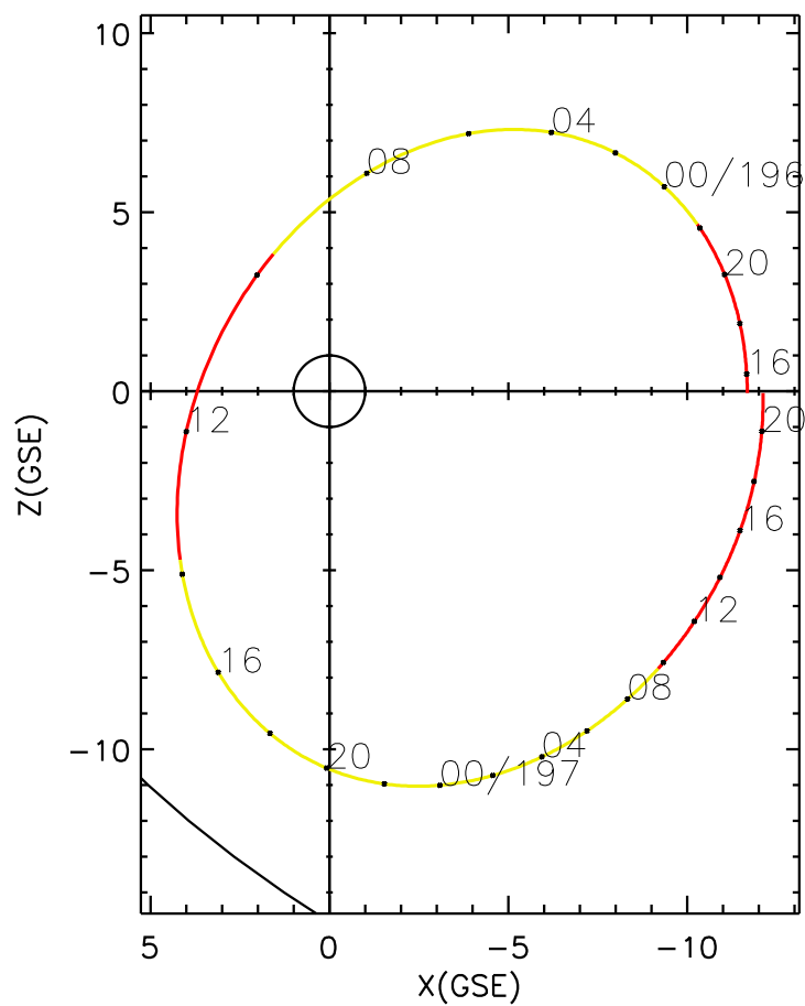
CLUSTER 2 orbit 2016 195 (07/13) 15:16 UT to 2016 197 (07/15) 21:31 UT
