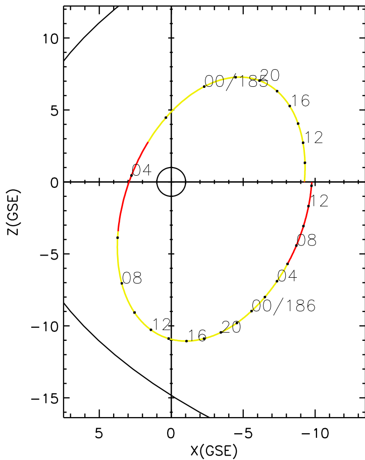
CLUSTER 2 orbit 2016 184 (07/02) 08:06 UT to 2016 186 (07/04) 14:21 UT
