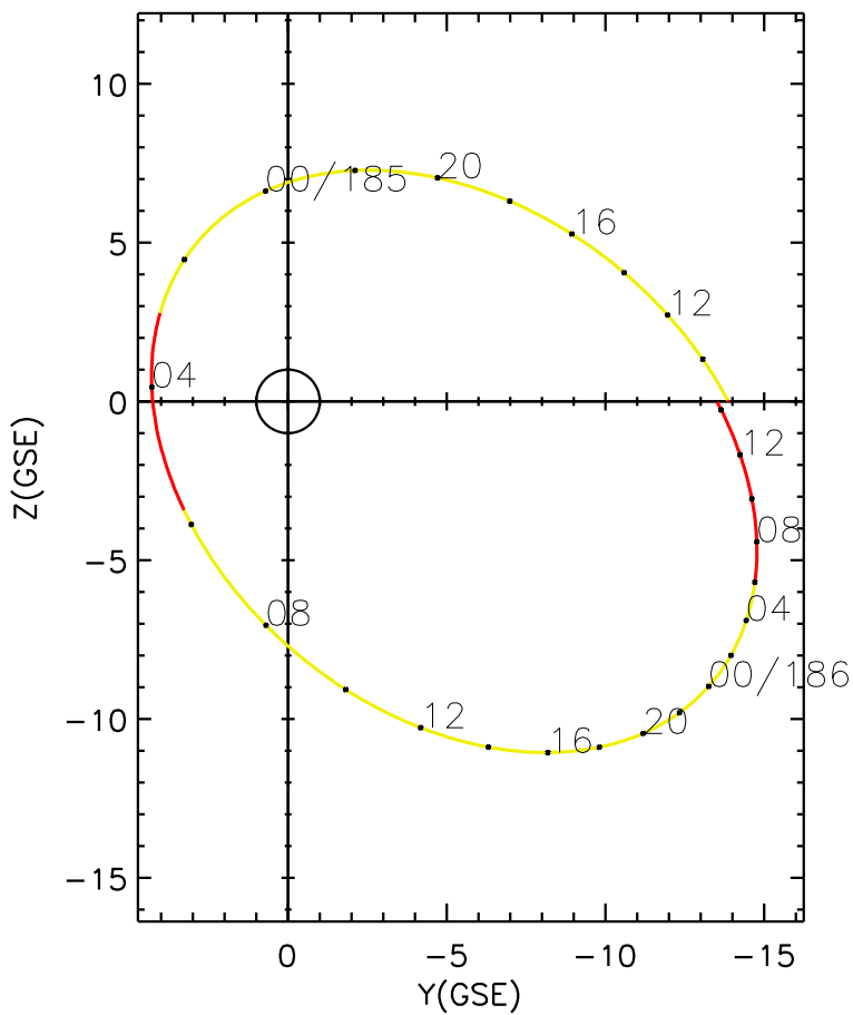
CLUSTER 2 orbit 2016 184 (07/02) 08:06 UT to 2016 186 (07/04) 14:21 UT
