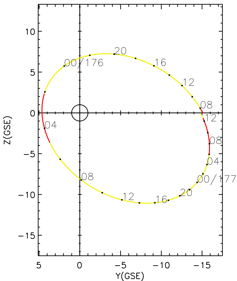
CLUSTER 2 orbit 2016 175 (06/23) 07:11 UT to 2016 177 (06/25) 13:21 UT
