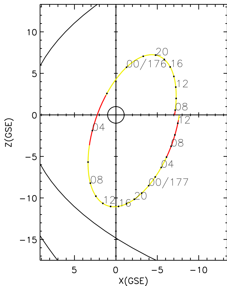
CLUSTER 2 orbit 2016 175 (06/23) 07:11 UT to 2016 177 (06/25) 13:21 UT
