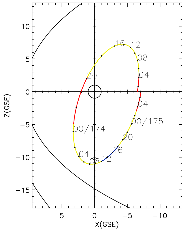
CLUSTER 2 orbit 2016 173 (06/21) 00:56 UT to 2016 175 (06/23) 07:11 UT
