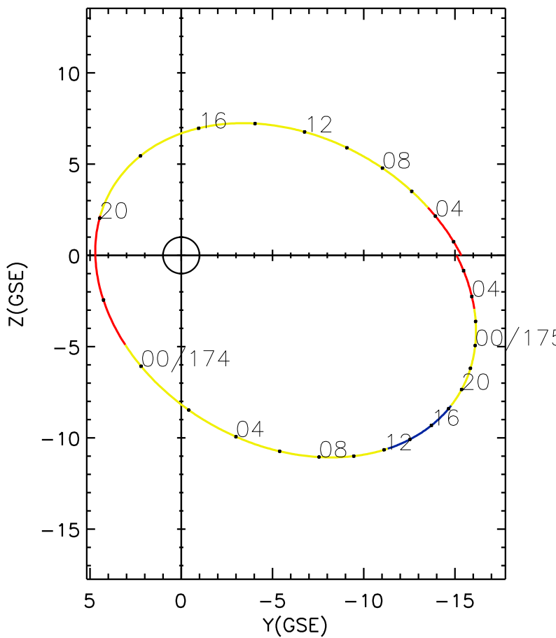
CLUSTER 2 orbit 2016 173 (06/21) 00:56 UT to 2016 175 (06/23) 07:11 UT
