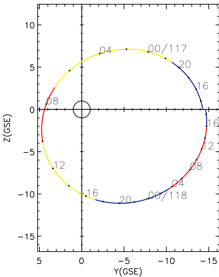
CLUSTER 2 orbit 2016 116 (04/25) 12:31 UT to 2016 118 (04/27) 18:46 UT
