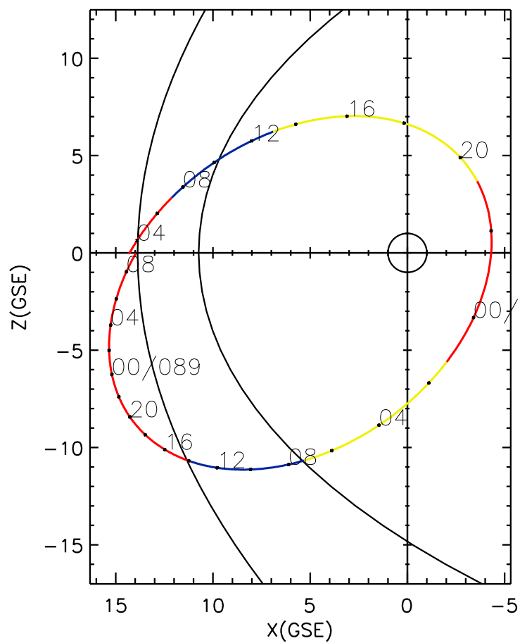
CLUSTER 2 orbit 2016 087 (03/27) 03:01 UT to 2016 089 (03/29) 09:21 UT
