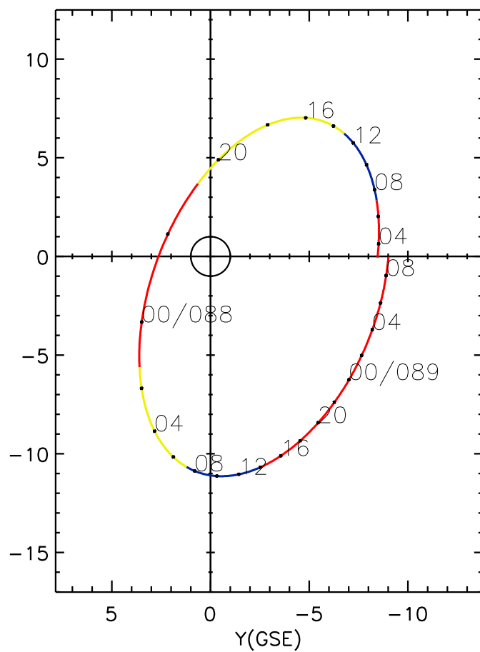
CLUSTER 2 orbit 2016 087 (03/27) 03:01 UT to 2016 089 (03/29) 09:21 UT
