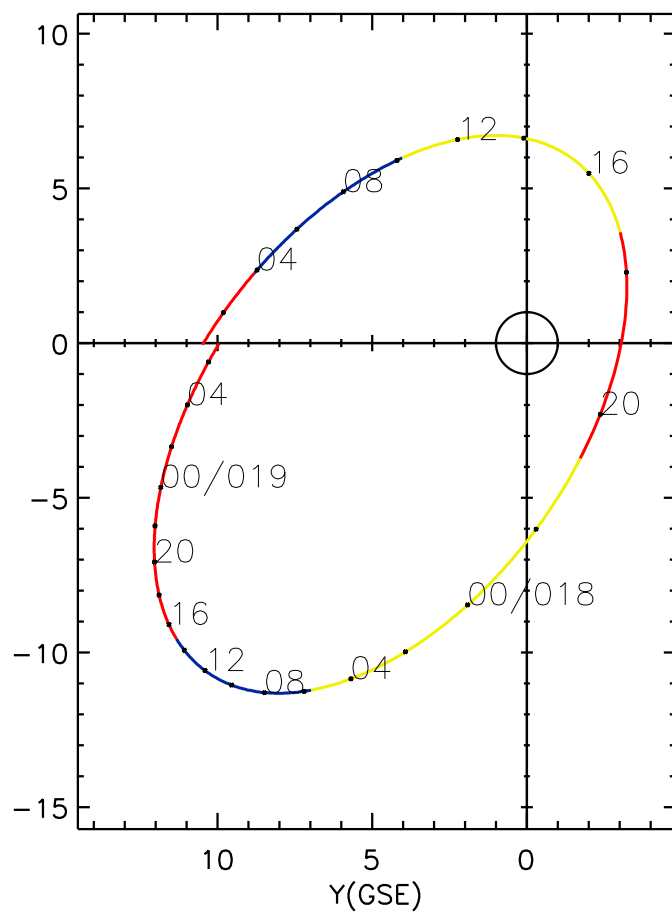
CLUSTER 2 orbit 2016 017 (01/17) 00:31 UT to 2016 019 (01/19) 06:51 UT
