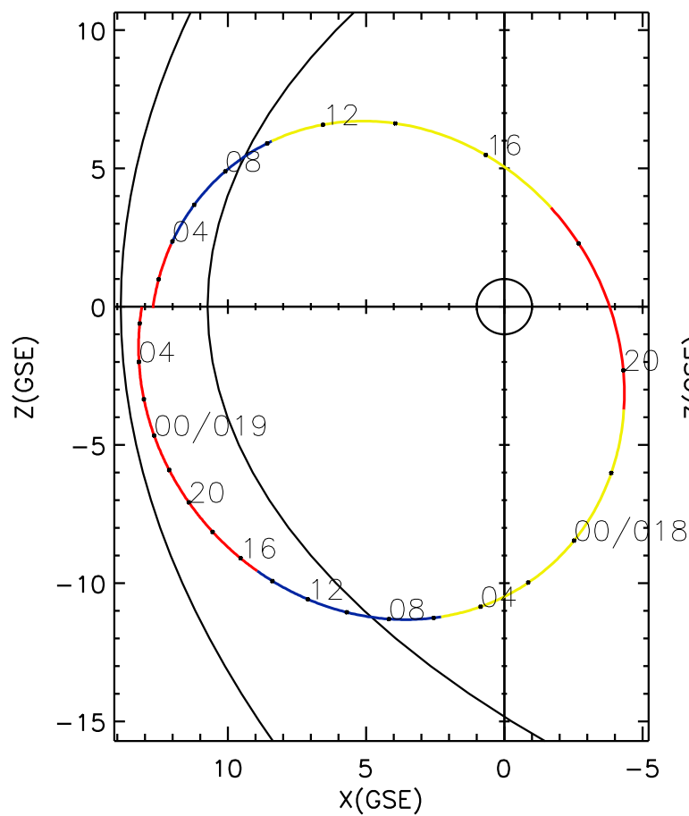
CLUSTER 2 orbit 2016 017 (01/17) 00:31 UT to 2016 019 (01/19) 06:51 UT
