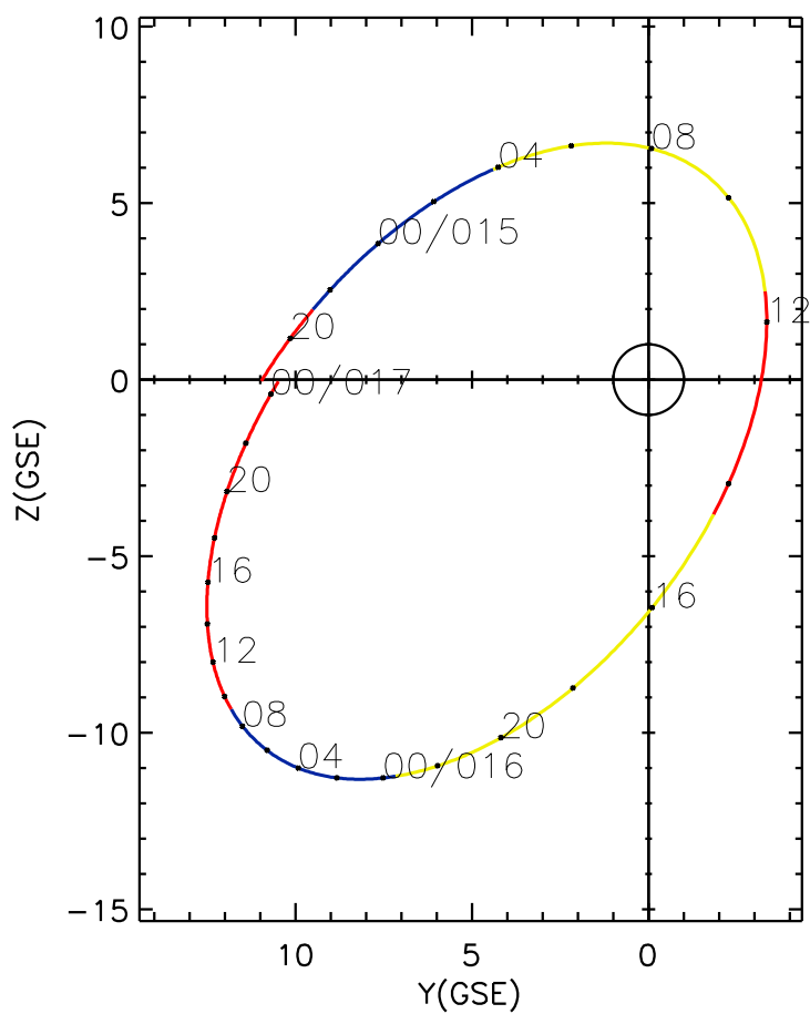
CLUSTER 2 orbit 2016 014 (01/14) 18:16 UT to 2016 017 (01/17) 00:31 UT
