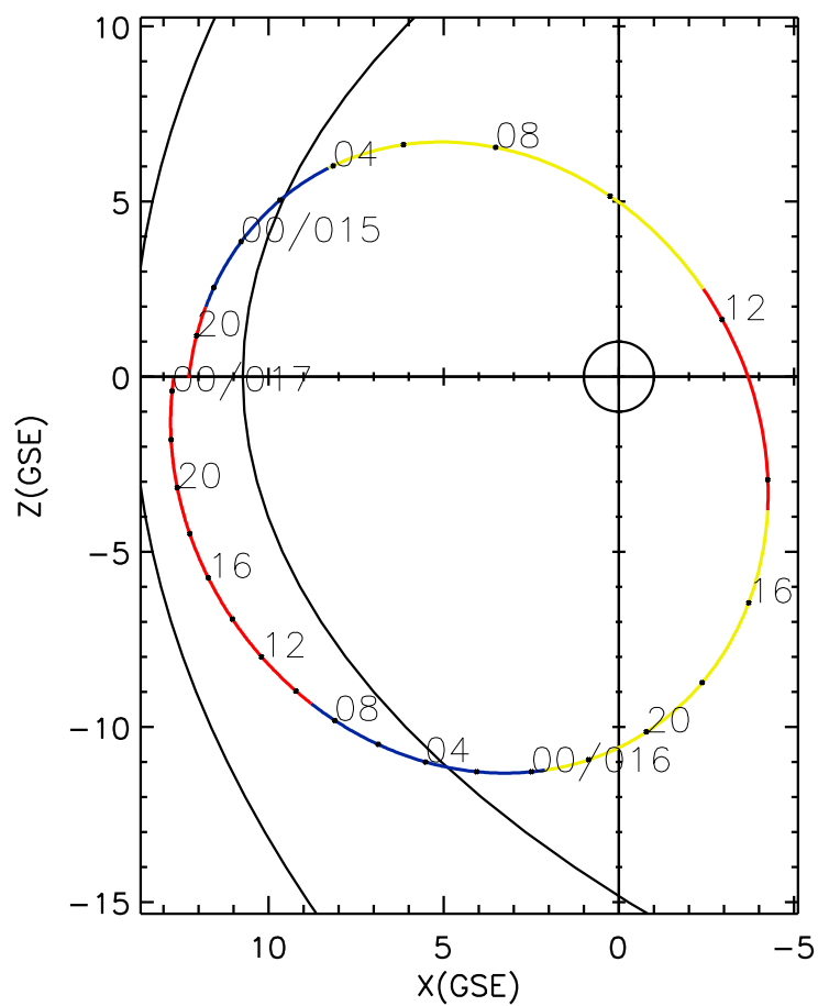
CLUSTER 2 orbit 2016 014 (01/14) 18:16 UT to 2016 017 (01/17) 00:31 UT
