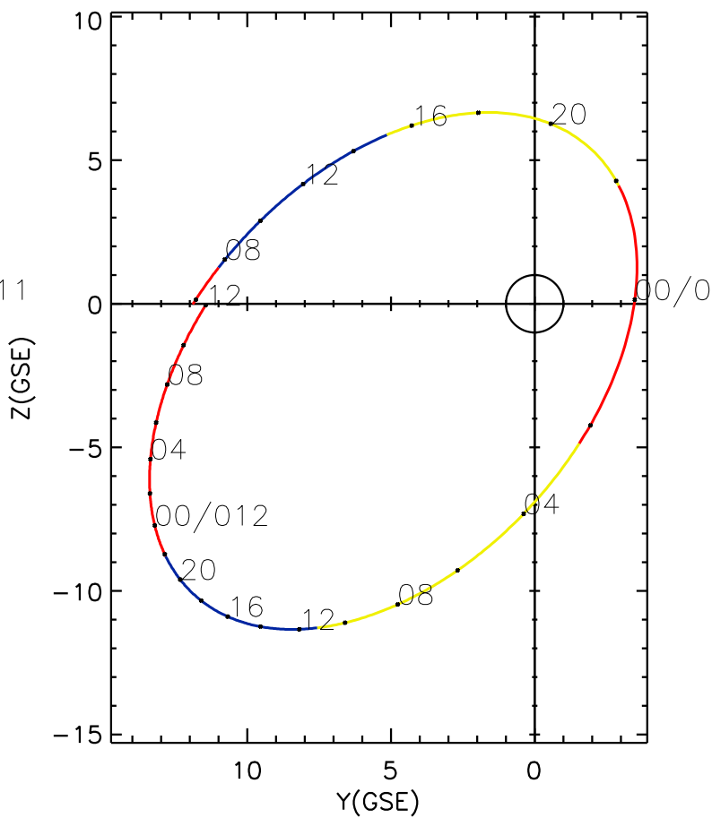
CLUSTER 2 orbit 2016 010 (01/10) 05:46 UT to 2016 012 (01/12) 12:01 UT
