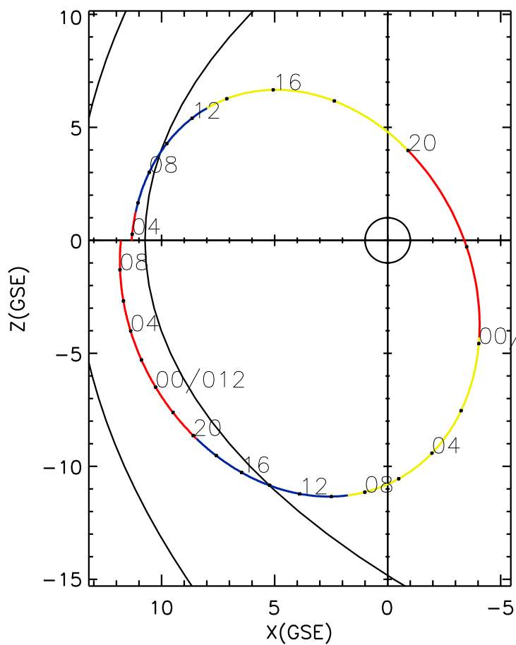
CLUSTER 2 orbit 2016 010 (01/10) 03:36 UT to 2016 012 (01/12) 09:51 UT
