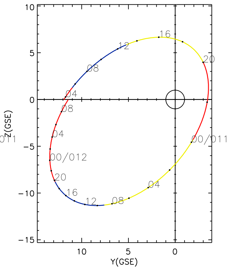
CLUSTER 2 orbit 2016 010 (01/10) 03:36 UT to 2016 012 (01/12) 09:51 UT
