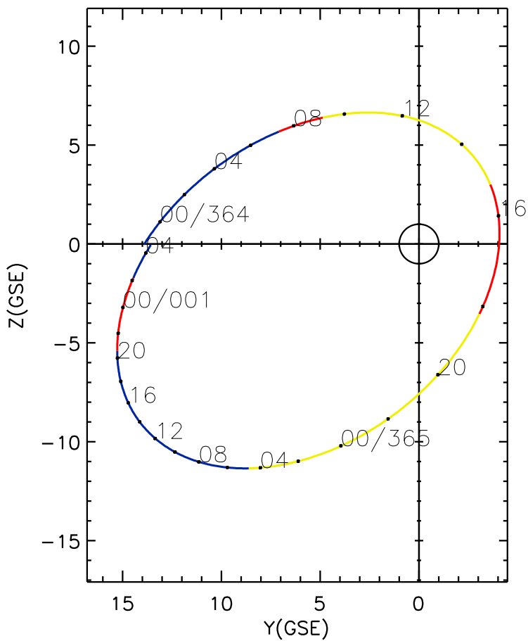
CLUSTER 2 orbit 2015 363 (12/29) 22:21 UT to 2016 001 (01/01) 04:36 UT
