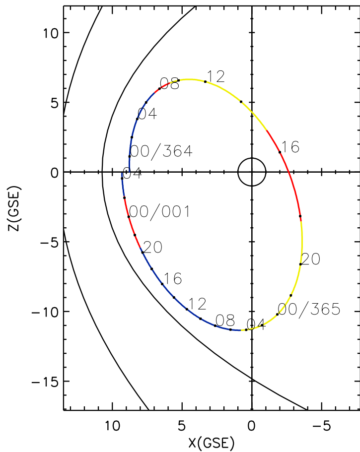
CLUSTER 2 orbit 2015 363 (12/29) 22:21 UT to 2016 001 (01/01) 04:36 UT
