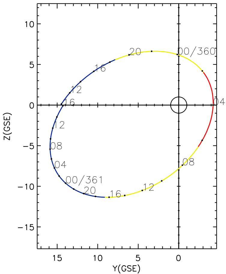
CLUSTER 2 orbit 2015 359 (12/25) 09:46 UT to 2015 361 (12/27) 16:06 UT
