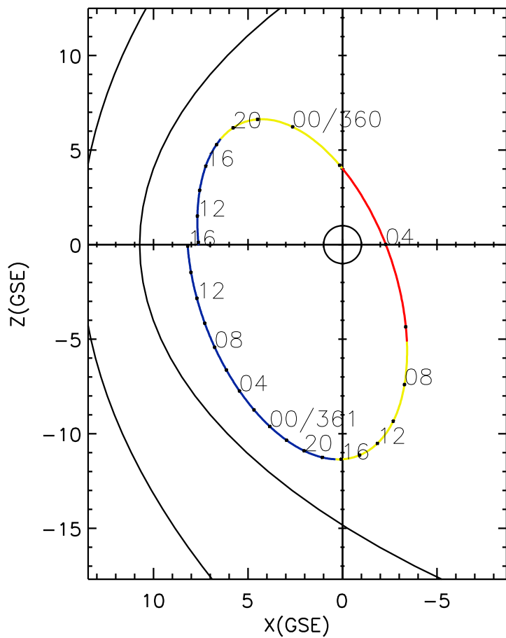
CLUSTER 2 orbit 2015 359 (12/25) 09:46 UT to 2015 361 (12/27) 16:06 UT
