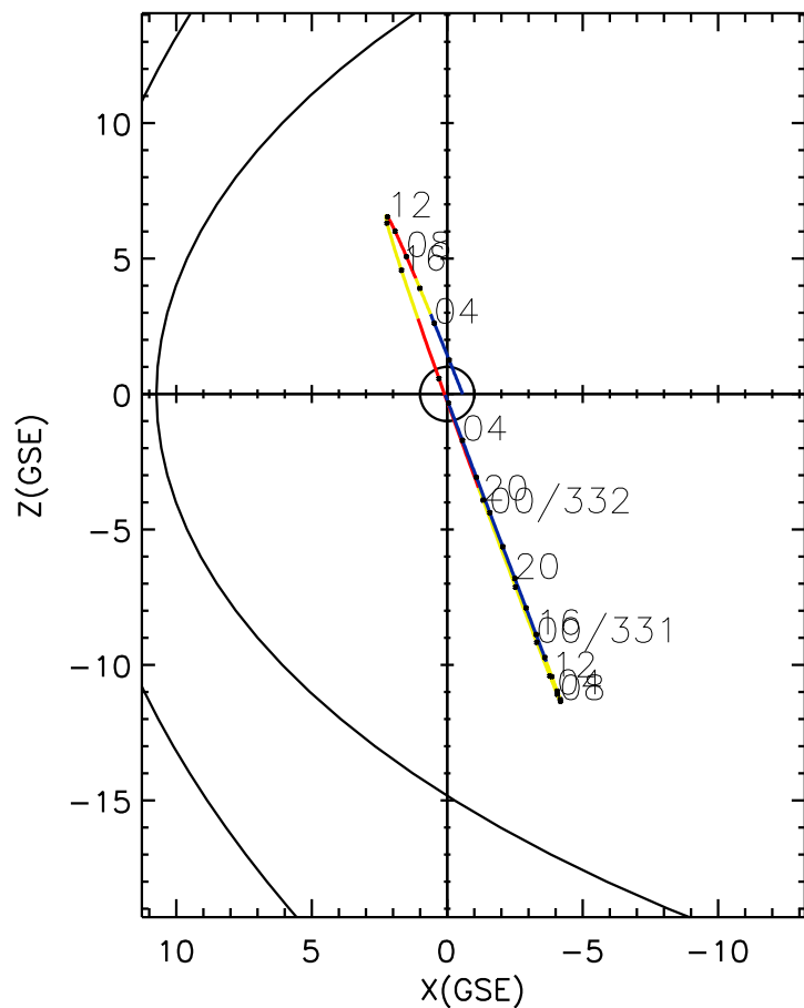
CLUSTER 2 orbit 2015 330 (11/26) 00:11 UT to 2015 332 (11/28) 06:26 UT
