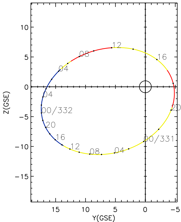
CLUSTER 2 orbit 2015 330 (11/26) 00:11 UT to 2015 332 (11/28) 06:26 UT
