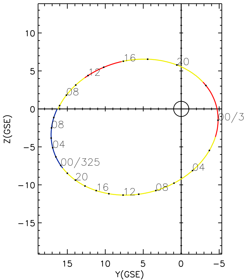
CLUSTER 2 orbit 2015 323 (11/19) 05:21 UT to 2015 325 (11/21) 11:36 UT
