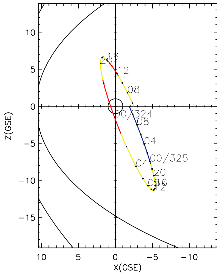
CLUSTER 2 orbit 2015 323 (11/19) 05:21 UT to 2015 325 (11/21) 11:36 UT
