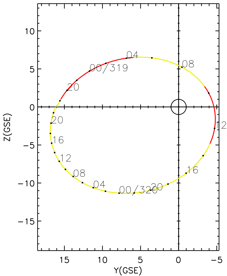
CLUSTER 2 orbit 2015 318 (11/14) 16:46 UT to 2015 320 (11/16) 23:06 UT
