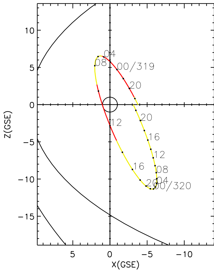
CLUSTER 2 orbit 2015 318 (11/14) 16:46 UT to 2015 320 (11/16) 23:06 UT
