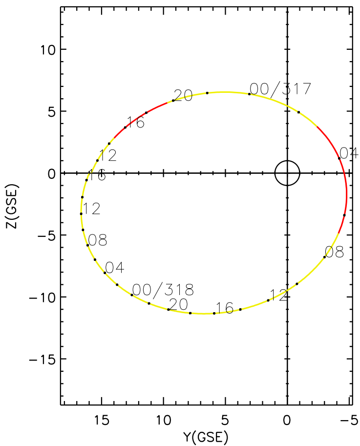
CLUSTER 2 orbit 2015 316 (11/12) 10:31 UT to 2015 318 (11/14) 16:46 UT
