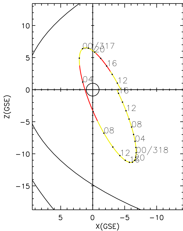
CLUSTER 2 orbit 2015 316 (11/12) 10:31 UT to 2015 318 (11/14) 16:46 UT
