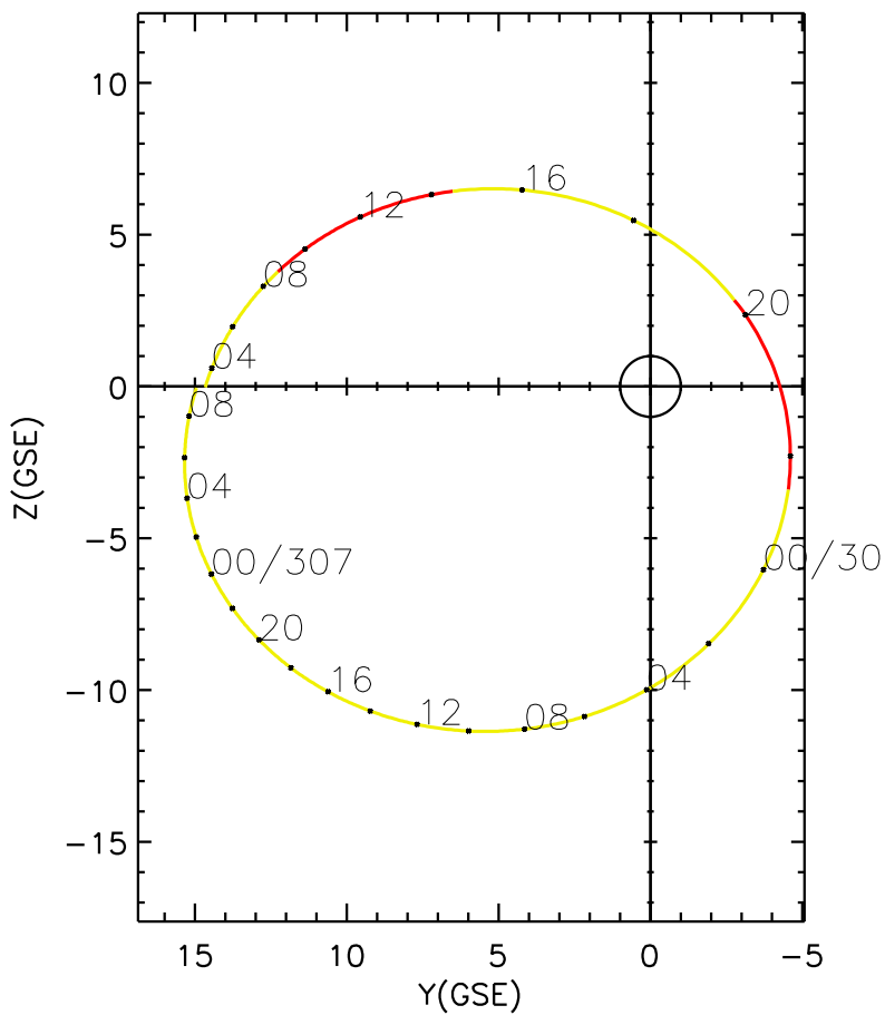
CLUSTER 2 orbit 2015 305 (11/01) 03:06 UT to 2015 307 (11/03) 09:21 UT
