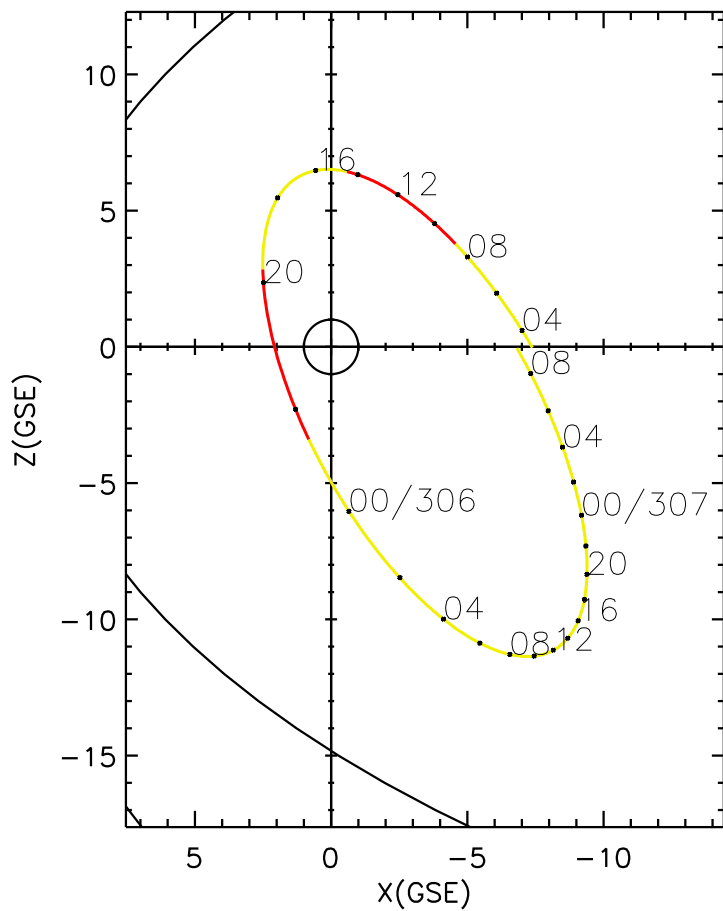
CLUSTER 2 orbit 2015 305 (11/01) 03:06 UT to 2015 307 (11/03) 09:21 UT
