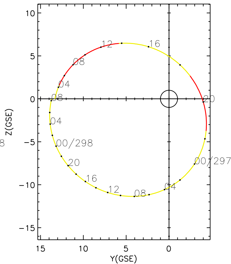
CLUSTER 2 orbit 2015 296 (10/23) 02:01 UT to 2015 298 (10/25) 08:16 UT
