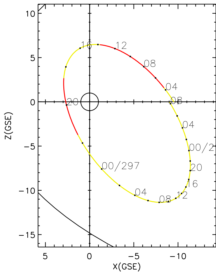
CLUSTER 2 orbit 2015 296 (10/23) 02:01 UT to 2015 298 (10/25) 08:16 UT
