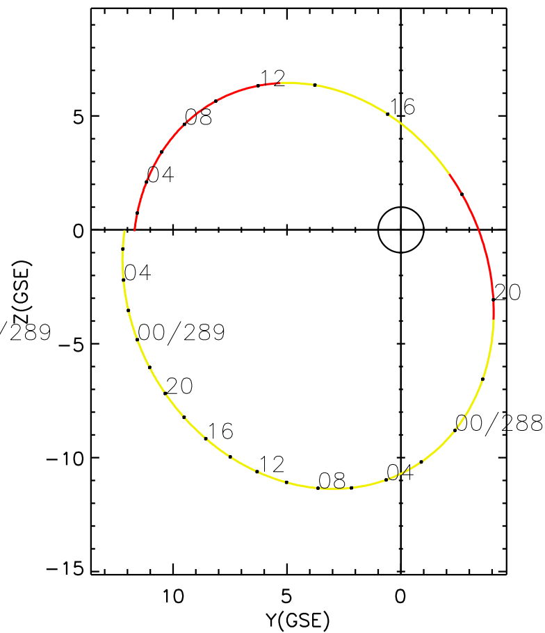
CLUSTER 2 orbit 2015 287 (10/14) 00:51 UT to 2015 289 (10/16) 07:11 UT
