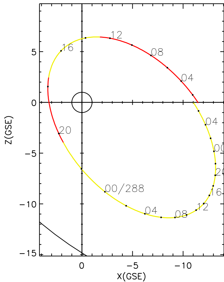
CLUSTER 2 orbit 2015 287 (10/14) 00:51 UT to 2015 289 (10/16) 07:11 UT
