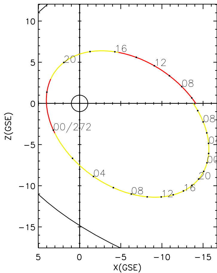
CLUSTER 2 orbit 2015 271 (09/28) 05:01 UT to 2015 273 (09/30) 11:16 UT
