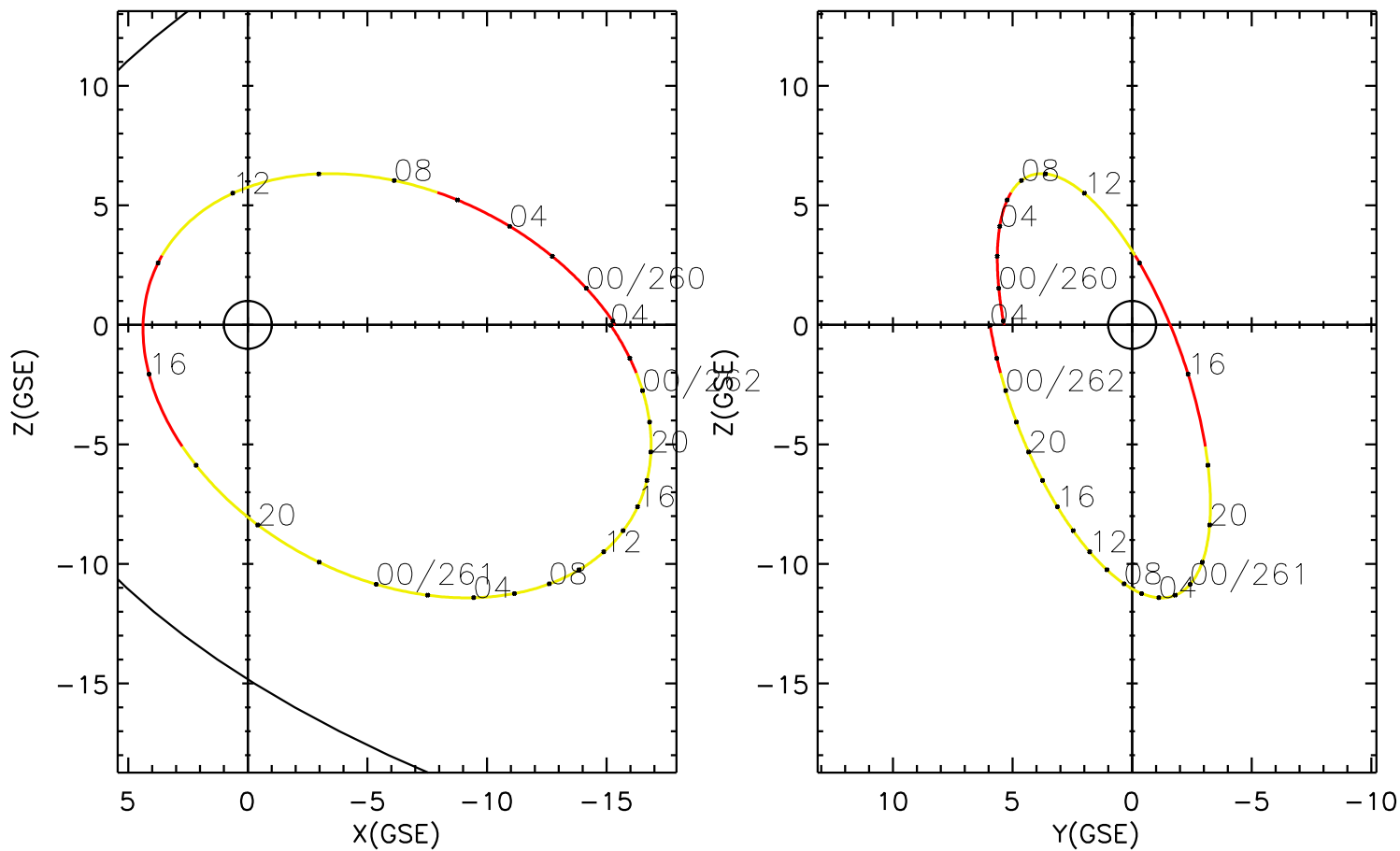
CLUSTER 2 orbit 2015 259 (09/16) 21:46 UT to 2015 262 (09/19) 04:01 UT
