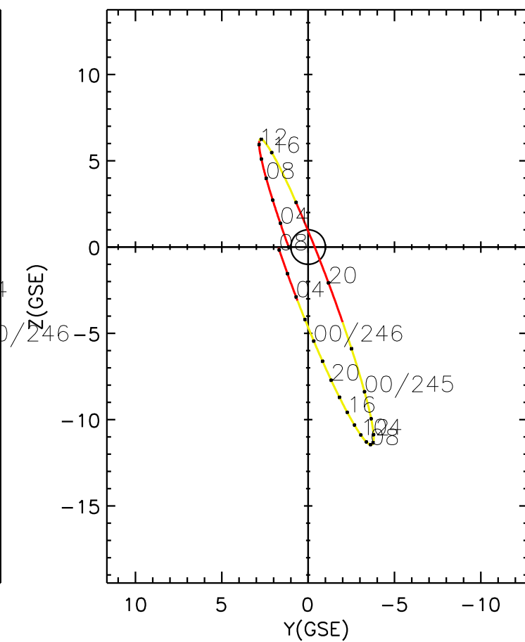
CLUSTER 2 orbit 2015 244 (09/01) 01:56 UT to 2015 246 (09/03) 08:11 UT
