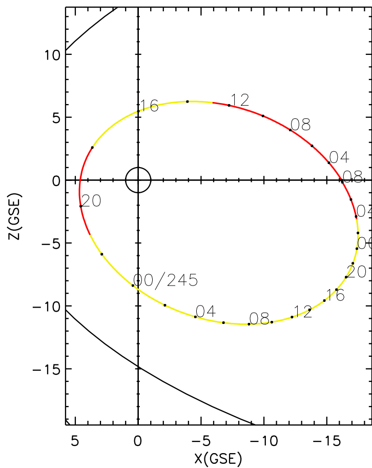
CLUSTER 2 orbit 2015 244 (09/01) 01:56 UT to 2015 246 (09/03) 08:11 UT
