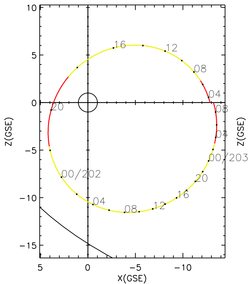
CLUSTER 2 orbit 2015 201 (07/20) 03:11 UT to 2015 203 (07/22) 09:26 UT
