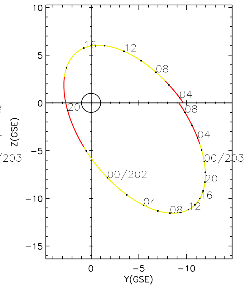
CLUSTER 2 orbit 2015 201 (07/20) 03:11 UT to 2015 203 (07/22) 09:26 UT
