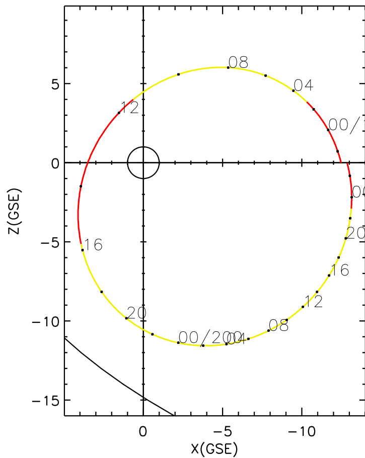
CLUSTER 2 orbit 2015 198 (07/17) 20:56 UT to 2015 201 (07/20) 03:11 UT
