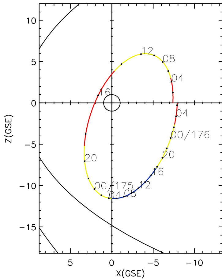
CLUSTER 2 orbit 2015 174 (06/23) 00:06 UT to 2015 176 (06/25) 06:21 UT
