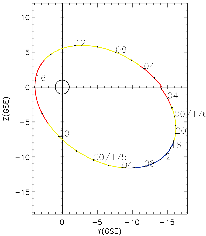
CLUSTER 2 orbit 2015 174 (06/23) 00:06 UT to 2015 176 (06/25) 06:21 UT
