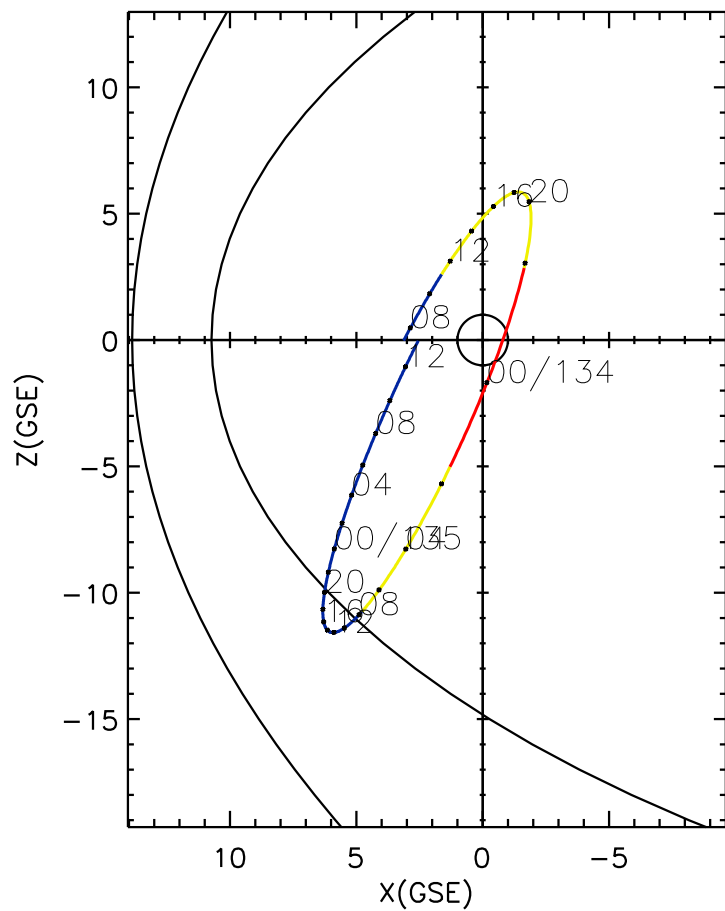
CLUSTER 2 orbit 2015 133 (05/13) 07:16 UT to 2015 135 (05/15) 13:31 UT
