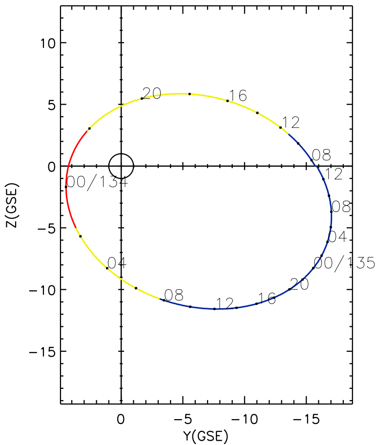
CLUSTER 2 orbit 2015 133 (05/13) 07:16 UT to 2015 135 (05/15) 13:31 UT
