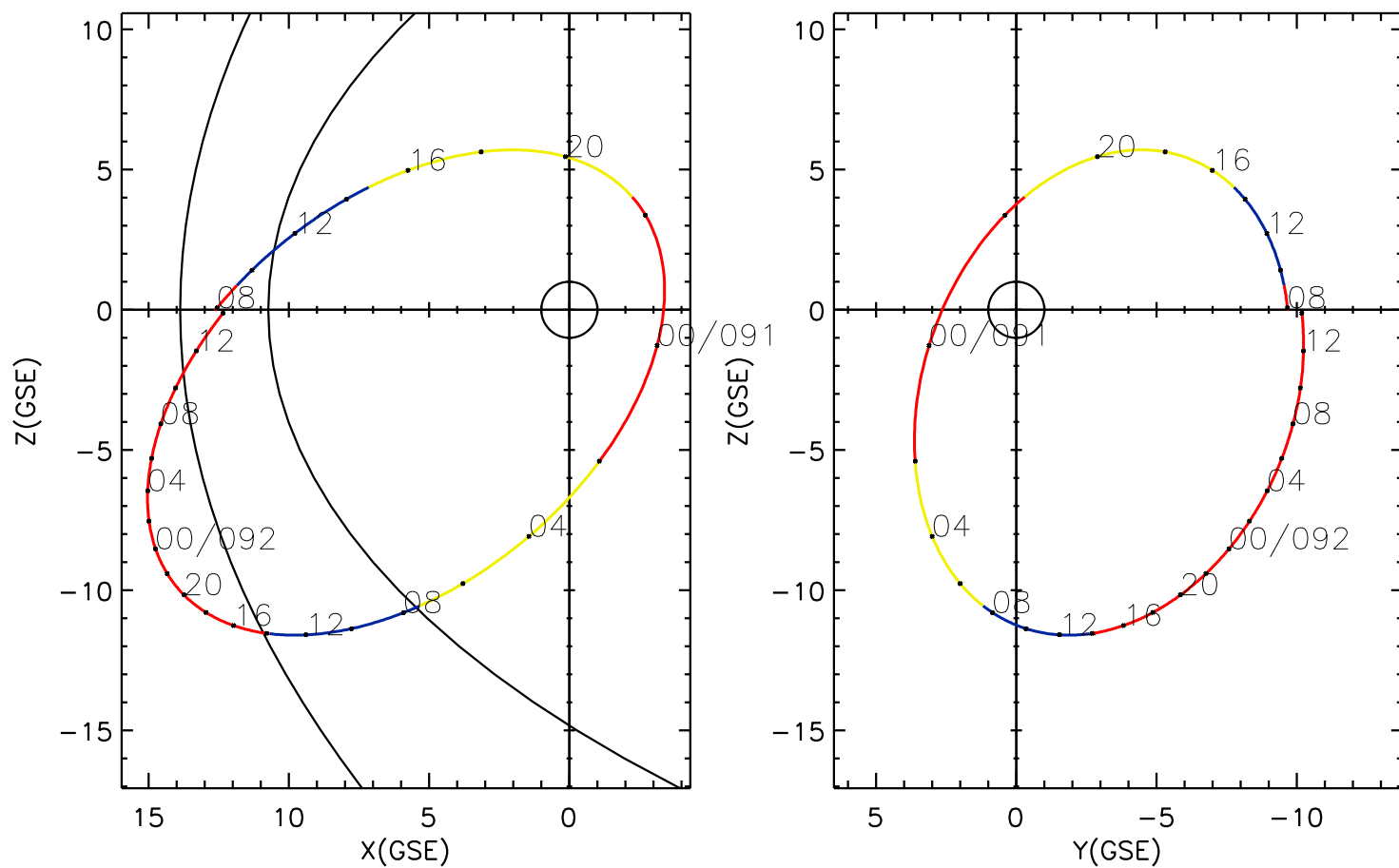
CLUSTER 2 orbit 2015 090 (03/31) 07:51 UT to 2015 092 (04/02) 14:06 UT
