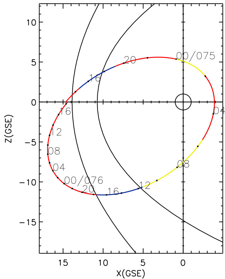
CLUSTER 2 orbit 2015 074 (03/15) 12:01 UT to 2015 076 (03/17) 18:16 UT
