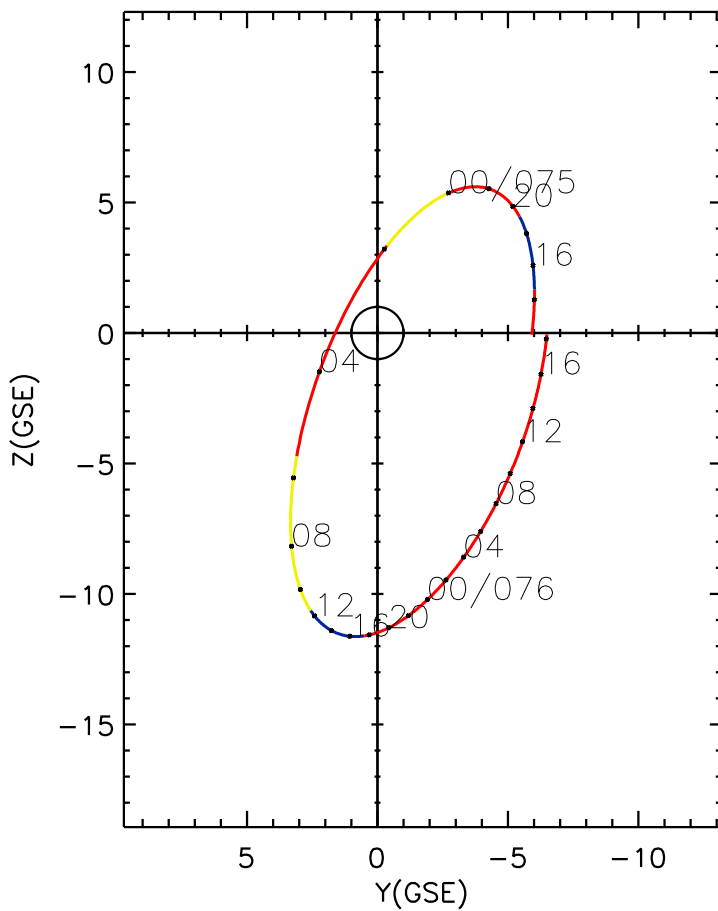
CLUSTER 2 orbit 2015 074 (03/15) 12:01 UT to 2015 076 (03/17) 18:16 UT
