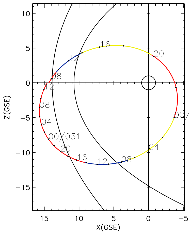
CLUSTER 2 orbit 2015 029 (01/29) 07:06 UT to 2015 031 (01/31) 13:21 UT
