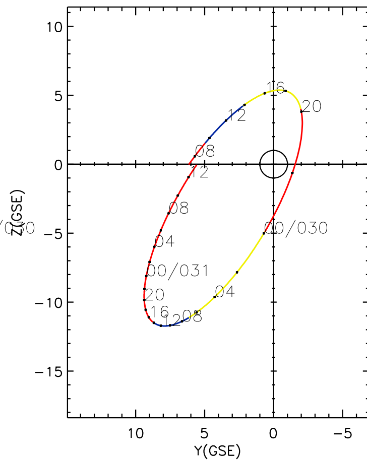
CLUSTER 2 orbit 2015 029 (01/29) 07:06 UT to 2015 031 (01/31) 13:21 UT
