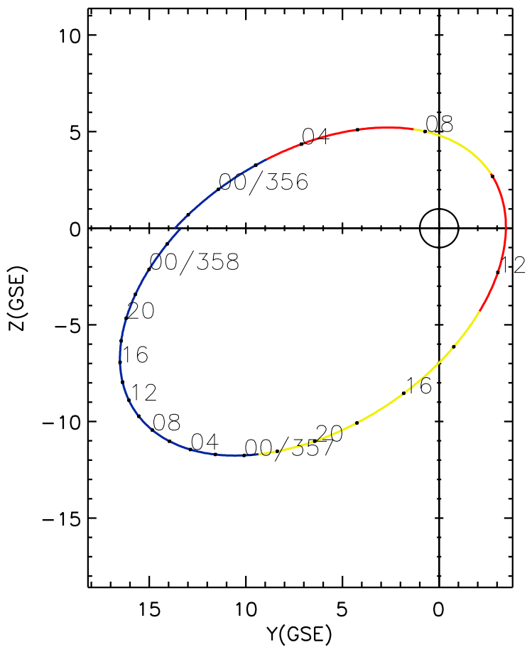
CLUSTER 2 orbit 2014 355 (12/21) 20:56 UT to 2014 358 (12/24) 03:11 UT
