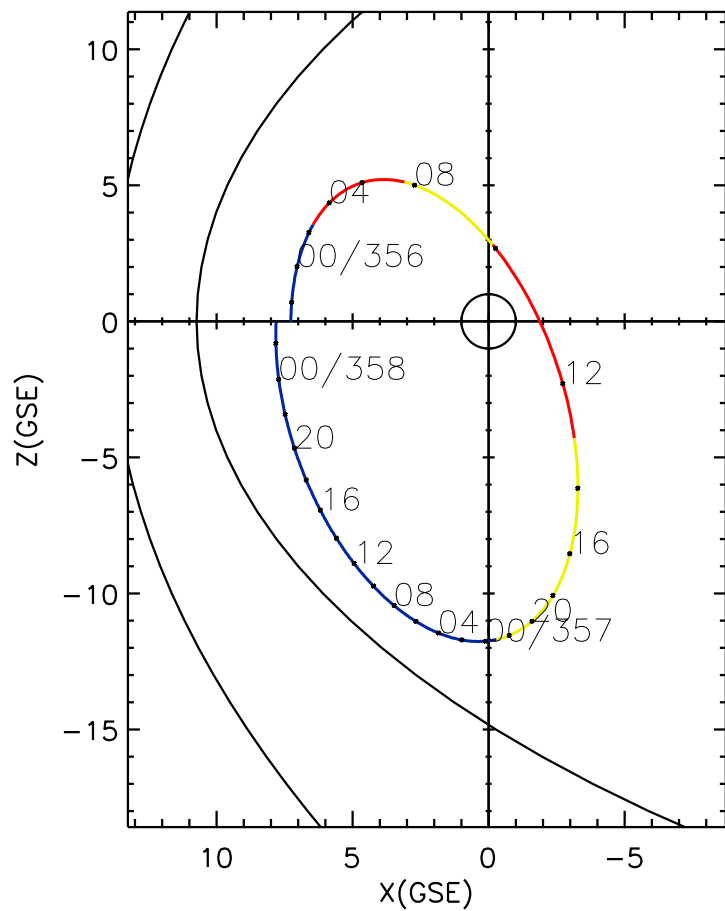
CLUSTER 2 orbit 2014 355 (12/21) 20:56 UT to 2014 358 (12/24) 03:11 UT
