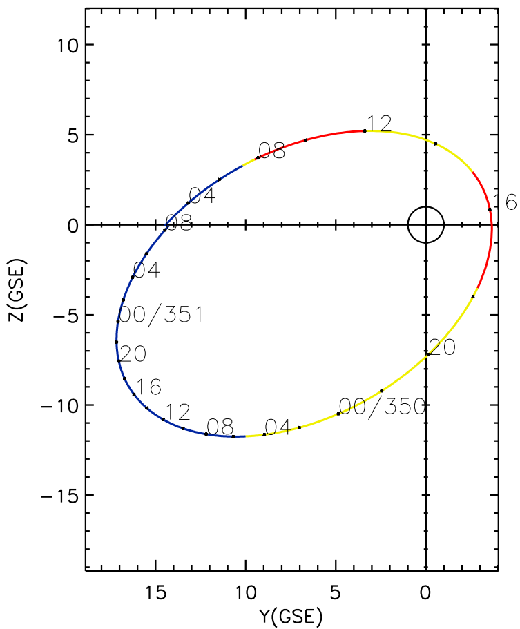
CLUSTER 2 orbit 2014 349 (12/15) 02:06 UT to 2014 351 (12/17) 08:21 UT
