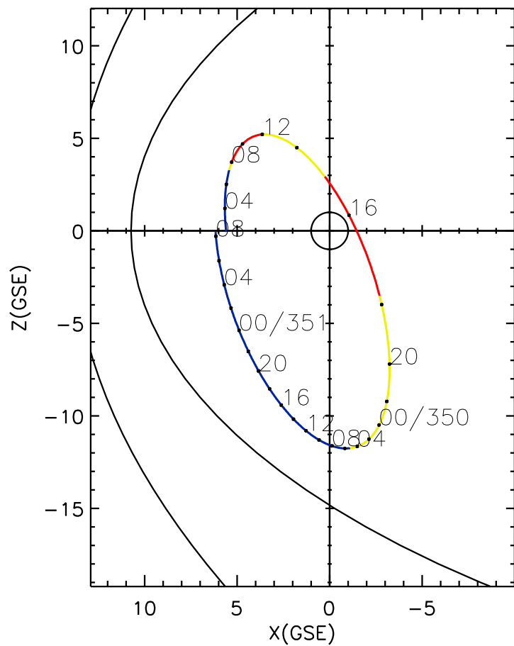
CLUSTER 2 orbit 2014 349 (12/15) 02:06 UT to 2014 351 (12/17) 08:21 UT
